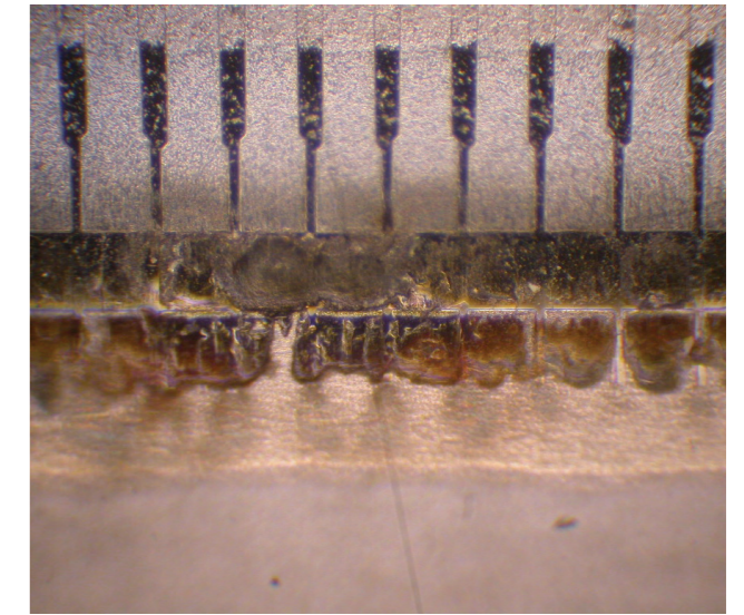
Pictures showing examples of printhead damage that can occur when using non-Zebra ribbons
